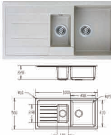
Model: DC-GS1005C Size: 1000x500mm Depth: 220mm
