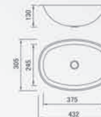
Model: DC-433 Size: 432x305mm Depth: 130mm
