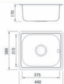
Model: DC-443 Size: 440x380mm Depth: 170mm
