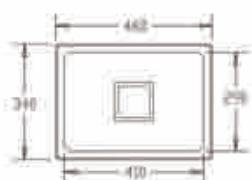
Model: DC-GS463S Size: 460x340mm Depth: 190mm
