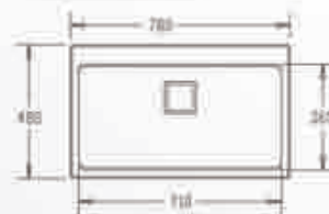
Model: DC-GS784BS Size: 780x480mm Depth: 210mm
