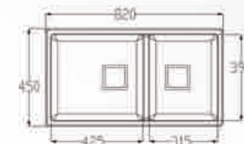
Model: DC-GS824S Size: 820x450mm Depth: 190mm
