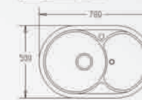
Model: DC-GS785 Size: 780x500mm Depth: 200mm
