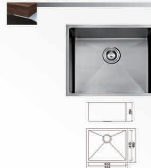
Model: DC-SR554 Size: 558x460mm Depth: 254mm Surface: Satin Thickness: 1.2mm Material: SUS304#
