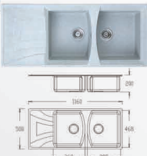
Model: DC-GS1165 Size: 1160x500mm Depth: 200mm
