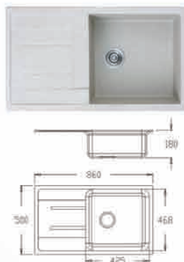
Model: DC-GS865E Size: 860x500mm Depth: 180mm
